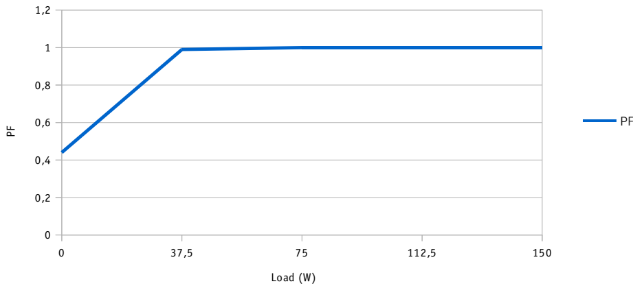
Power Factor versus Load 115V 400PHz
