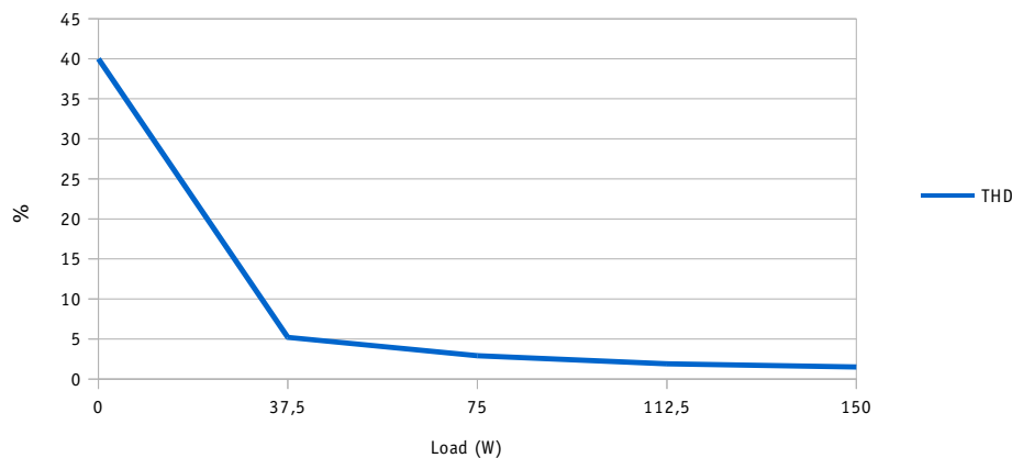
Total Harmonic Distortion (THD) versus Load at 115V 400Hz
